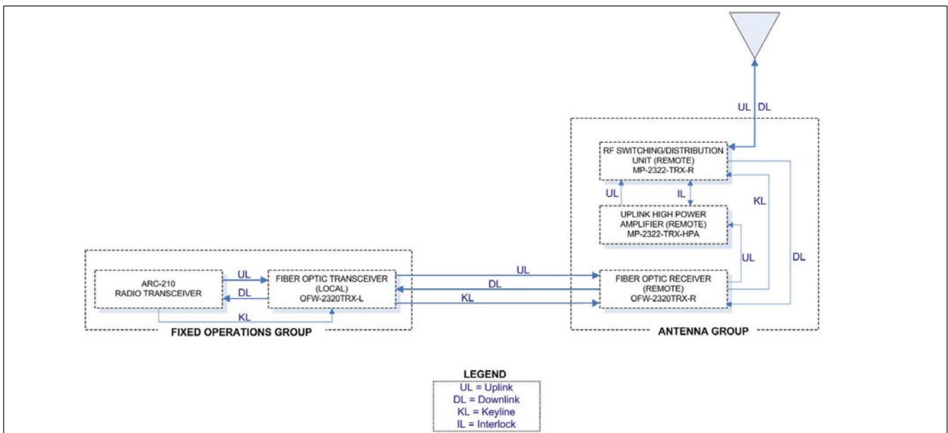
Tactical Radio Deployment - Function Block Diagram
